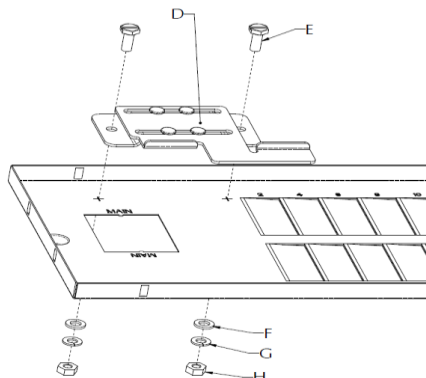
FIG. 3 Interlock Installation
