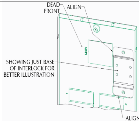
FIG. 2: Mounting Holes Location On the right side of Main
