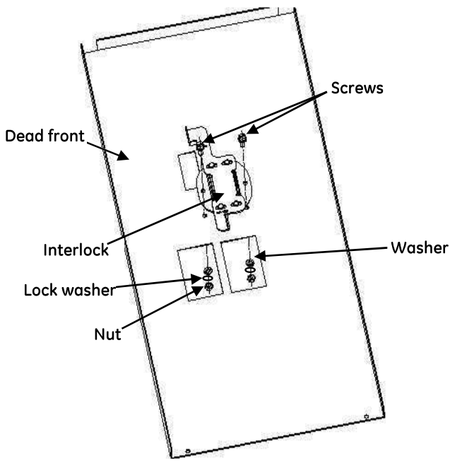
Figure 3: Interlock Installation
