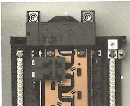
FIG. 1 Breaker Alignment
