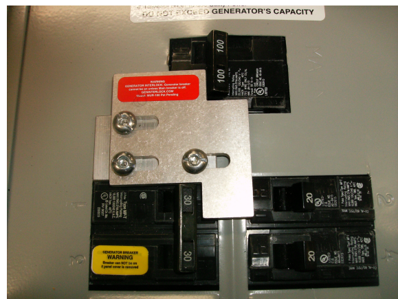
Generator On
