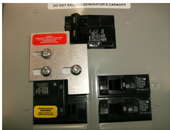
Main On
