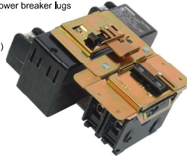
Fig. A Standby Power Main Breaker Incoming Utility Service Utility Main Breaker
