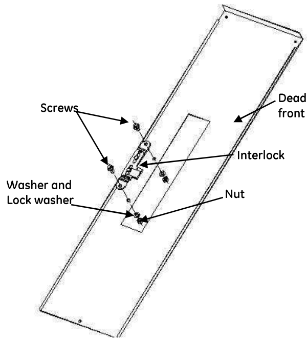
Figure 3: Interlock Installation
