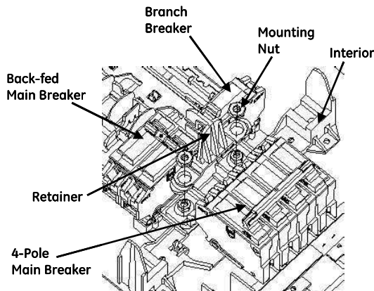
Figure 1: Main Breaker Retainer
